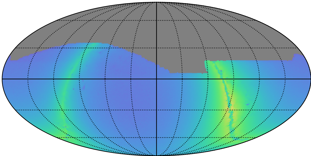
mw_roll_bulge_v3.3_10yrs i: Nstars_no_crowding
