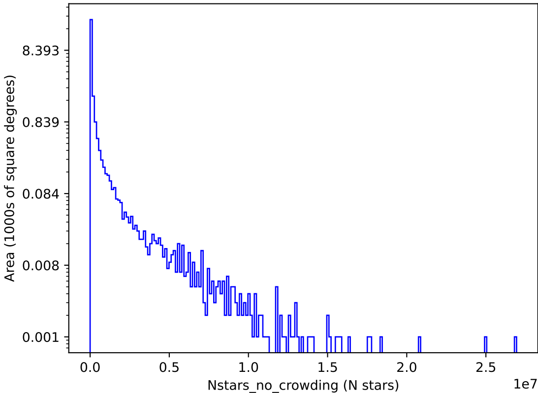
mw_roll_bulge_v3.3_10yrs i: Nstars_no_crowding
