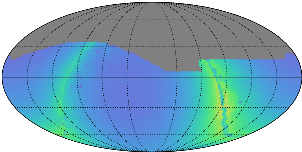
mw_roll_bulge_v3.3_10yrs g: Nstars_no_crowding
