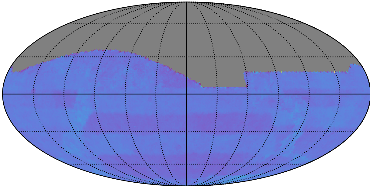
mw_roll_bulge_v3.3_10yrs : Normalized Proper Motion Uncert @ 24.0
