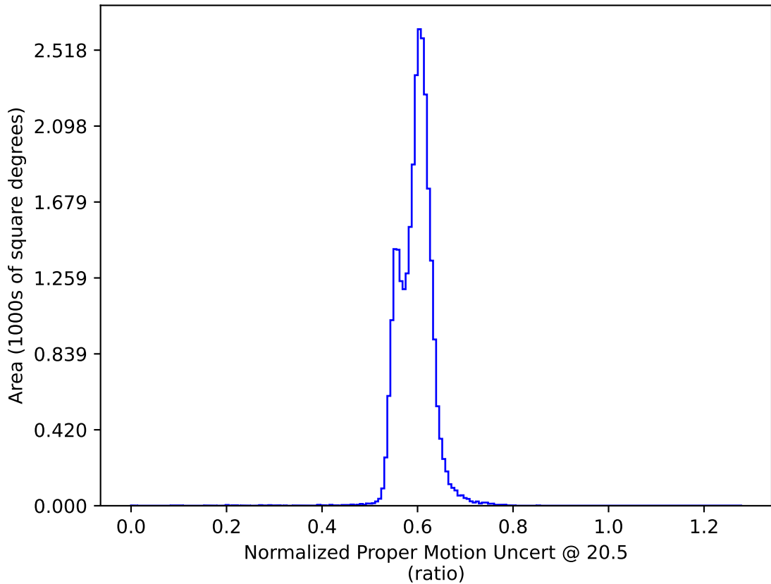
mw_roll_bulge_v3.3_10yrs : Normalized Proper Motion Uncert @ 20.5
