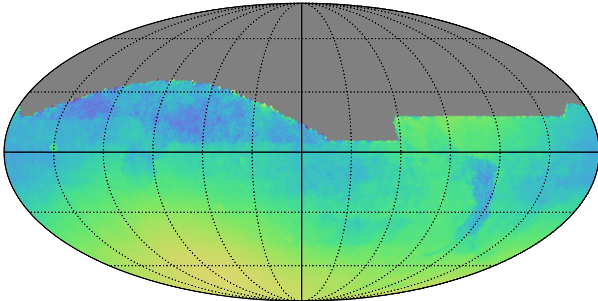
mw_roll_bulge_v3.3_10yrs : Normalized Parallax Uncert @ 24.0
