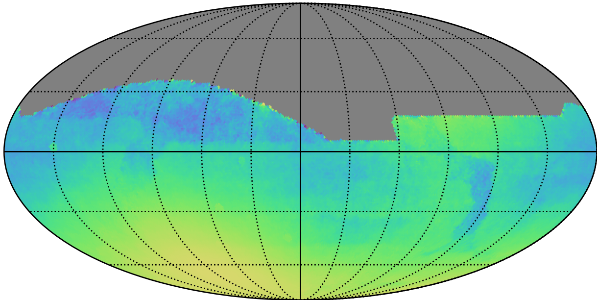
mw_roll_bulge_v3.3_10yrs : Normalized Parallax Uncert @ 22.4
