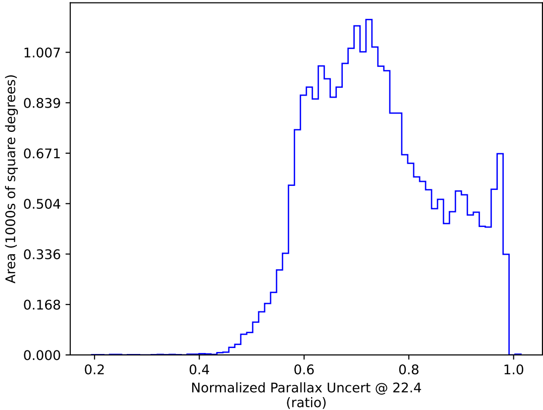
mw_roll_bulge_v3.3_10yrs : Normalized Parallax Uncert @ 22.4
