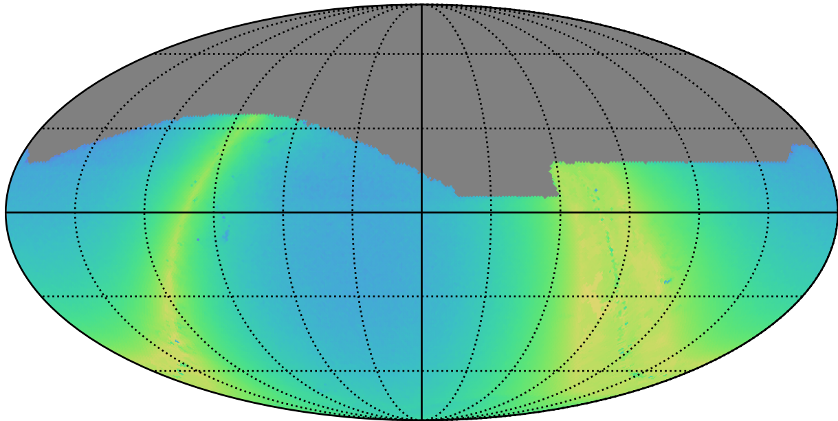
mw_roll_bulge_v3.3_10yrs z: N stars to Precision 0.20
