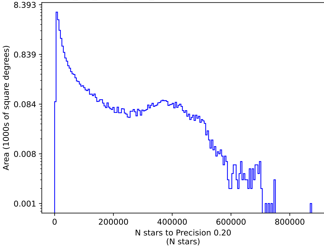
mw_roll_bulge_v3.3_10yrs z: N stars to Precision 0.20
