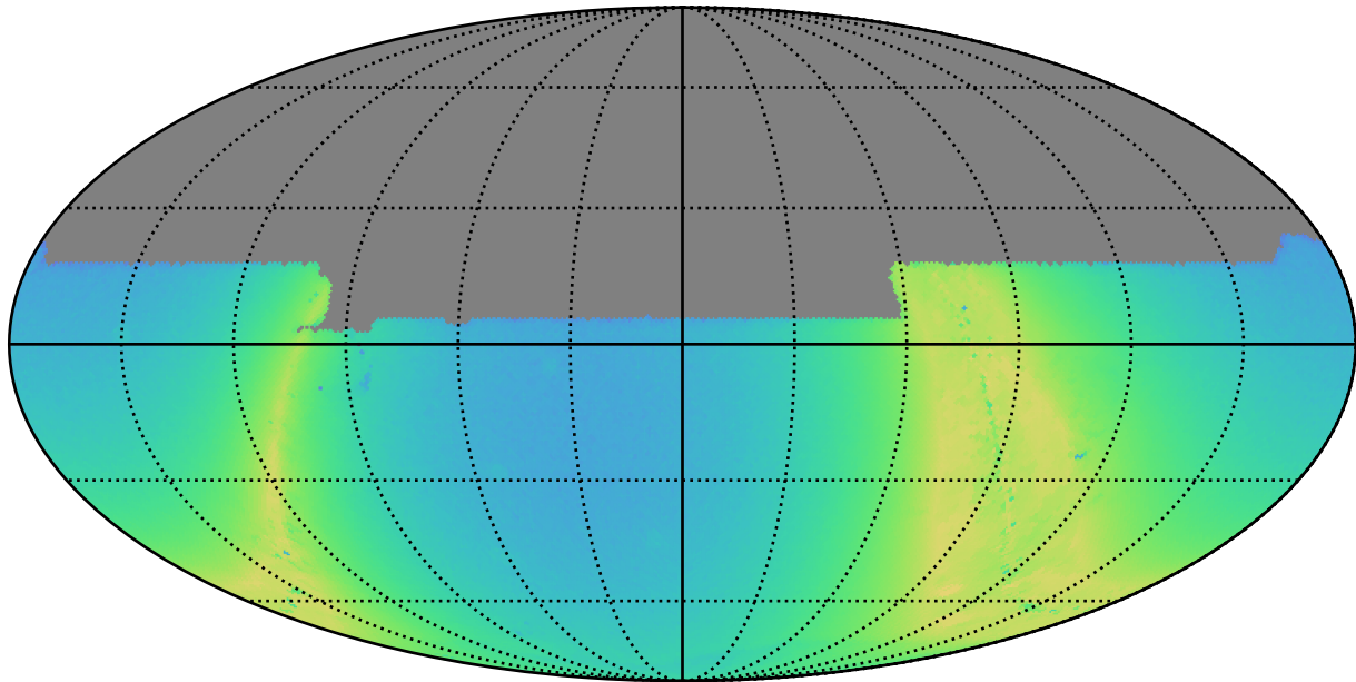
mw_roll_bulge_v3.3_10yrs y: N stars to Precision 0.20
