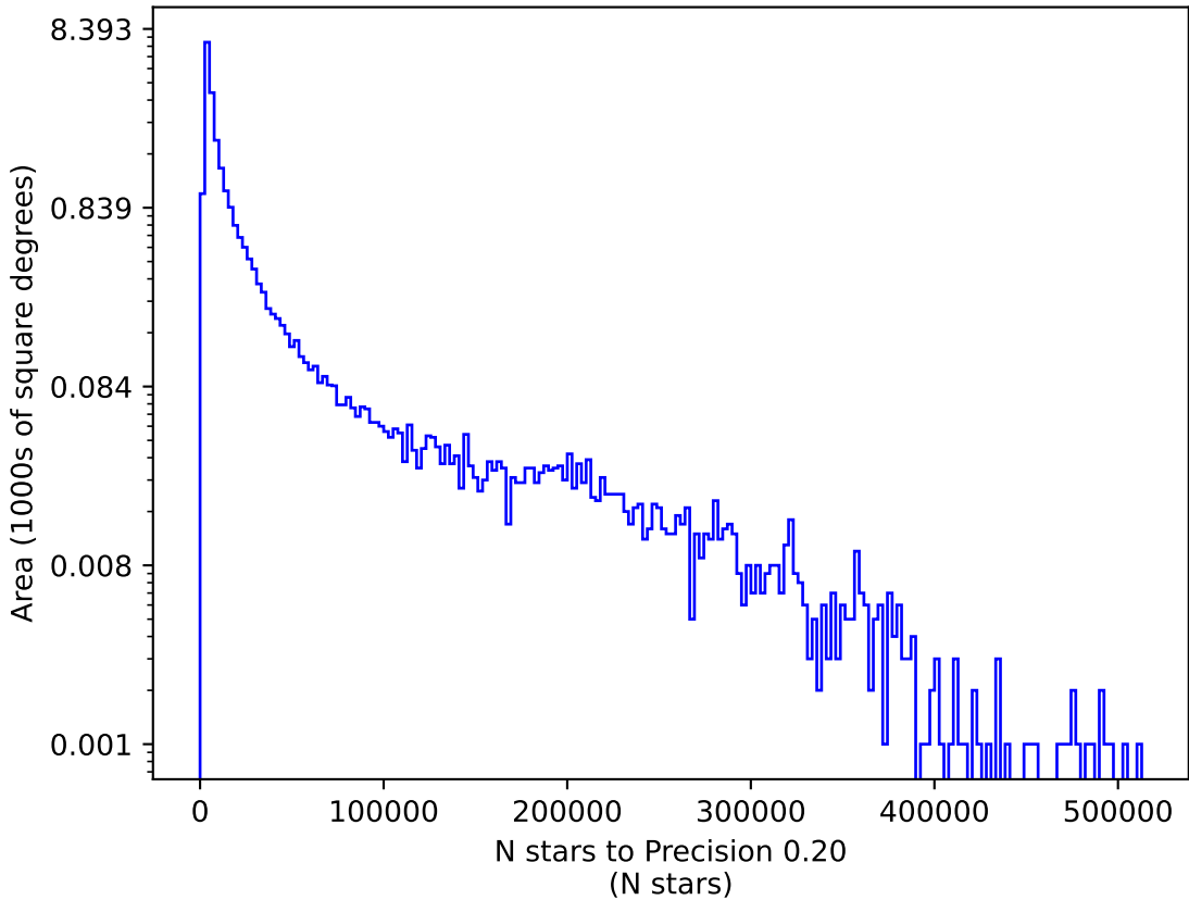
mw_roll_bulge_v3.3_10yrs u: N stars to Precision 0.20
