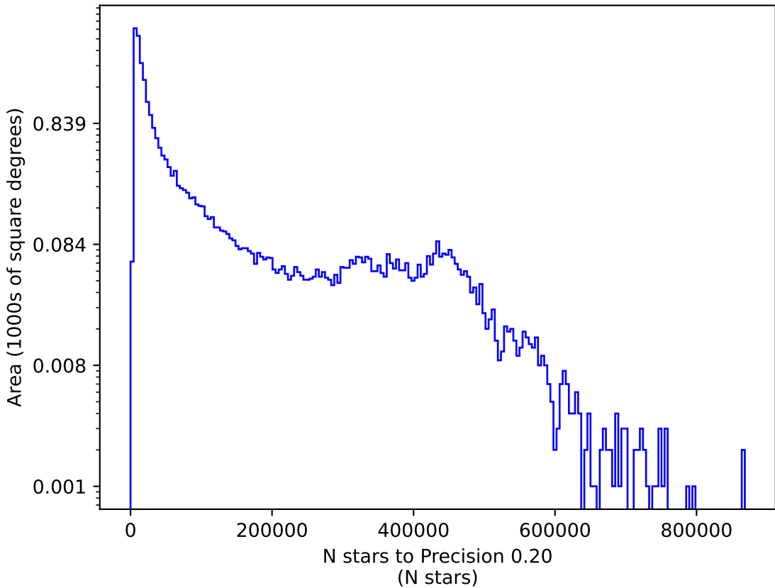
mw_roll_bulge_v3.3_10yrs r: N stars to Precision 0.20
