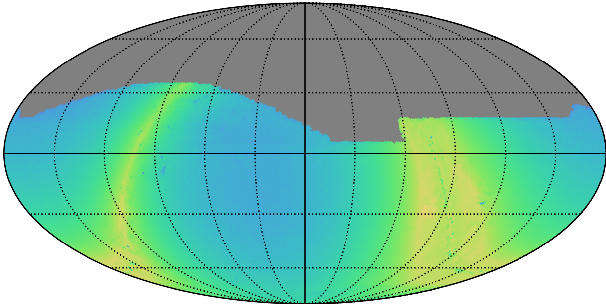
mw_roll_bulge_v3.3_10yrs i: N stars to Precision 0.20
