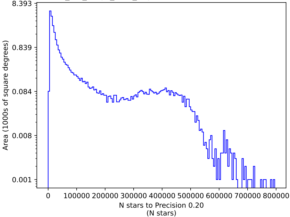
mw_roll_bulge_v3.3_10yrs i: N stars to Precision 0.20
