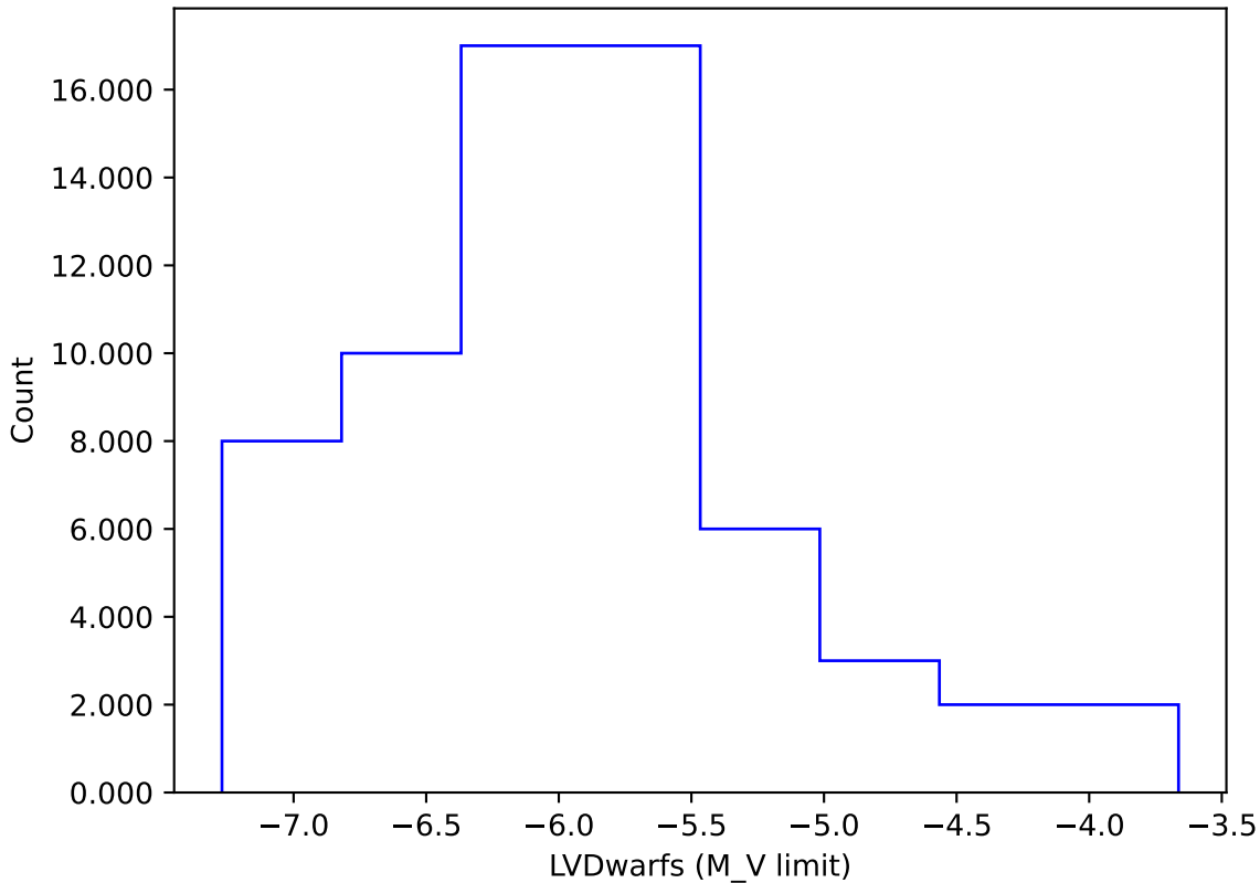
mw_roll_bulge_v3.3_10yrs gi: LVDwarfs
