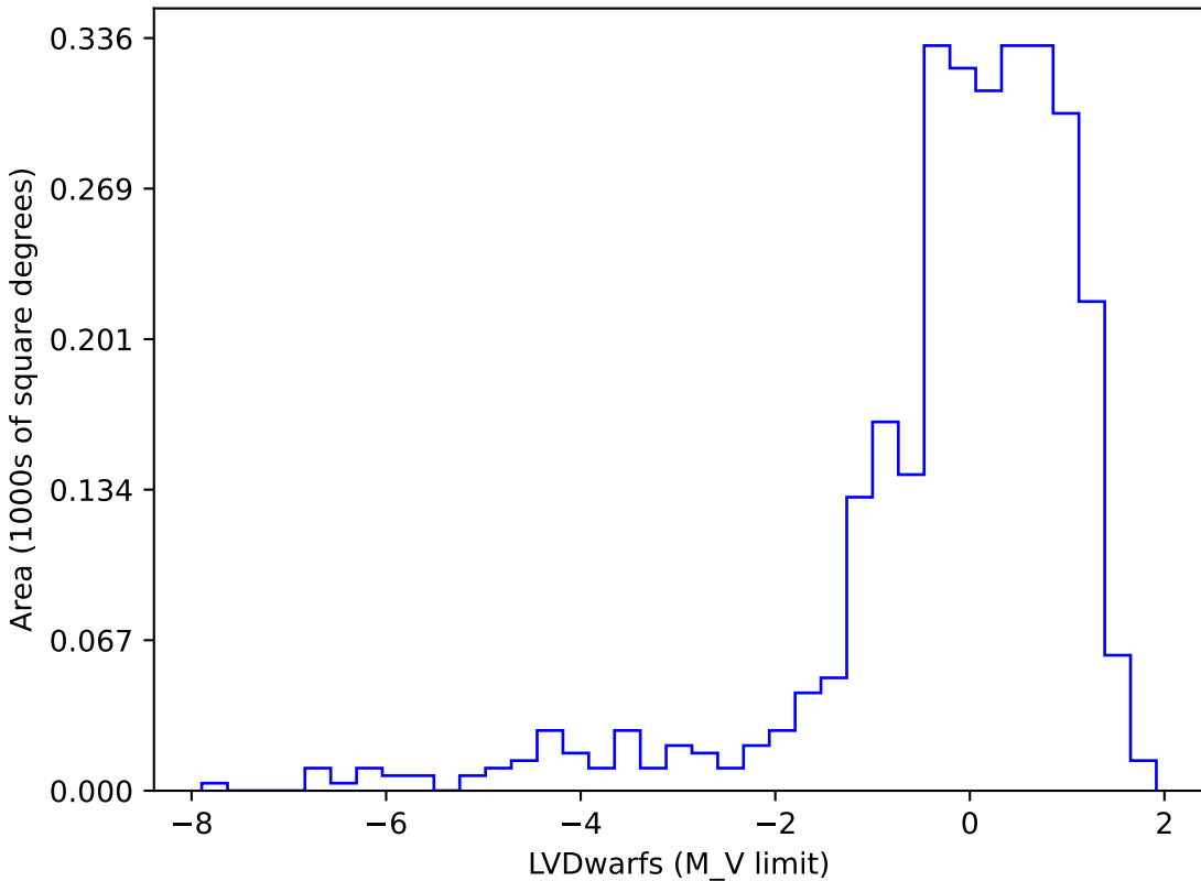
mw_roll_bulge_v3.3_10yrs gi SCP: LVDwarfs
