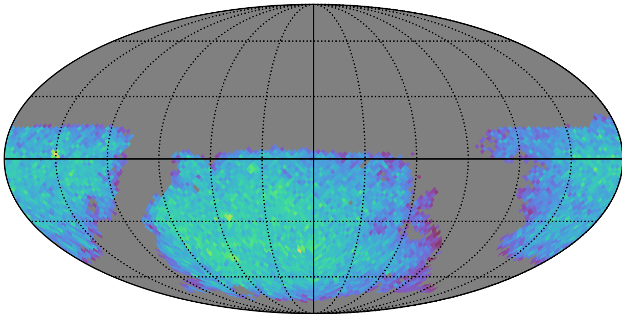
mw_roll_bulge_v3.3_10yrs gi: LVDwarfs
