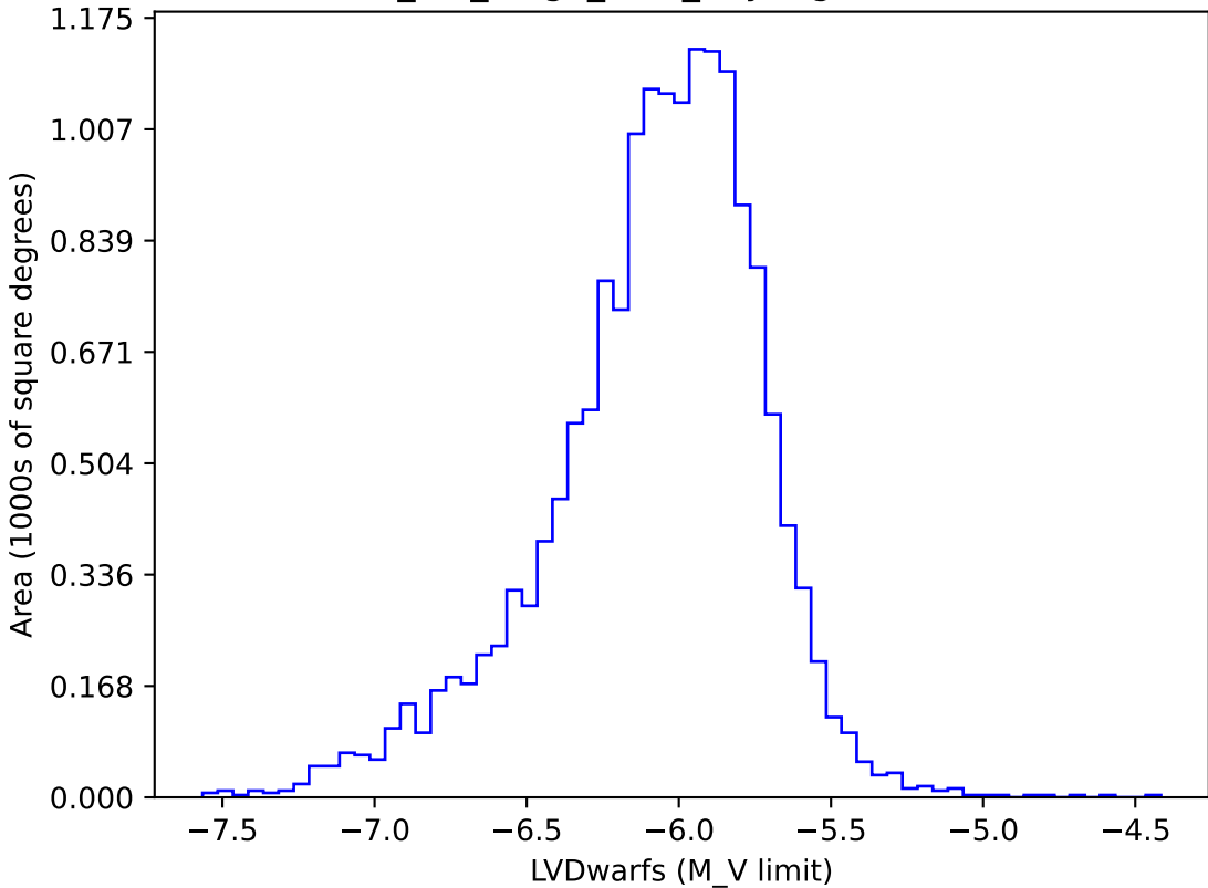
mw_roll_bulge_v3.3_10yrs gi: LVDwarfs
