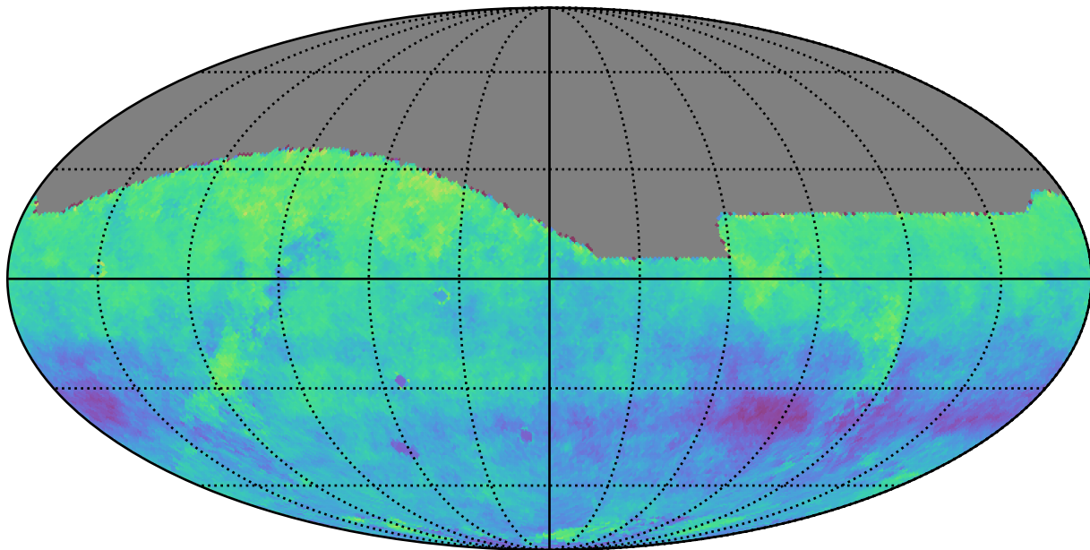
mw_roll_bulge_v3.3_10yrs z: Kuiper rotSkyPos
