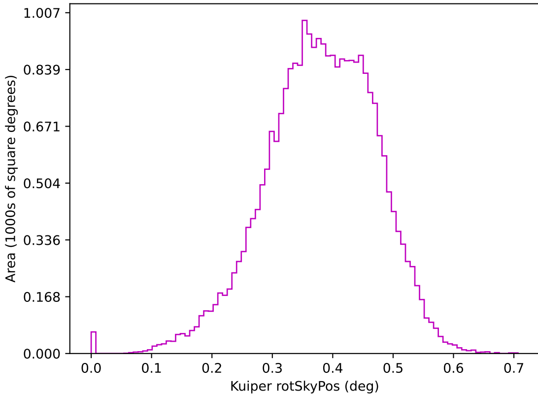
mw_roll_bulge_v3.3_10yrs z: Kuiper rotSkyPos
