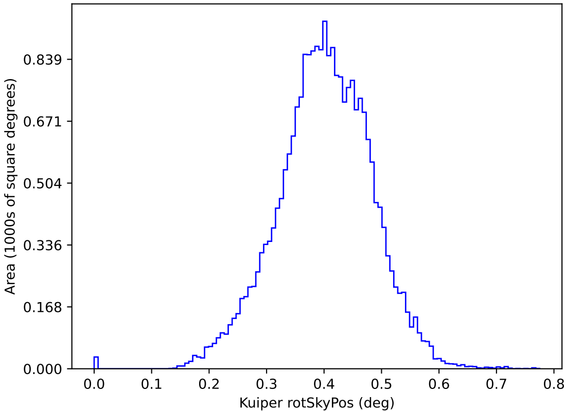
mw_roll_bulge_v3.3_10yrs y: Kuiper rotSkyPos
