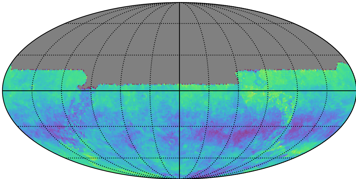
mw_roll_bulge_v3.3_10yrs u: Kuiper rotSkyPos
