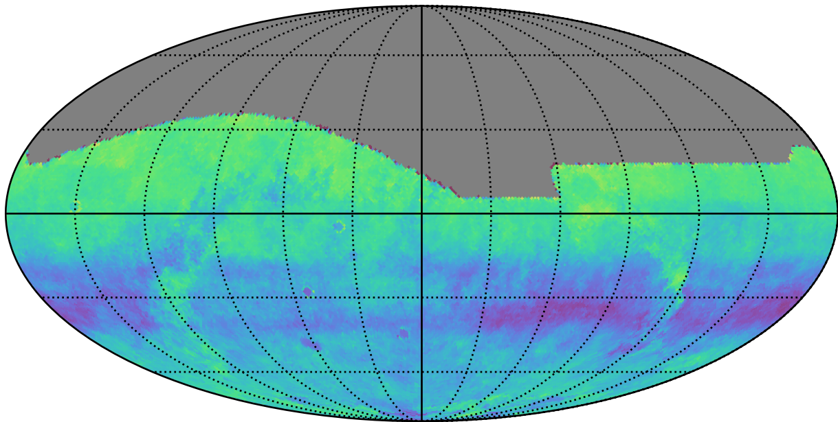
mw_roll_bulge_v3.3_10yrs r: Kuiper rotSkyPos
