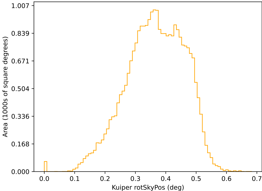
mw_roll_bulge_v3.3_10yrs r: Kuiper rotSkyPos
