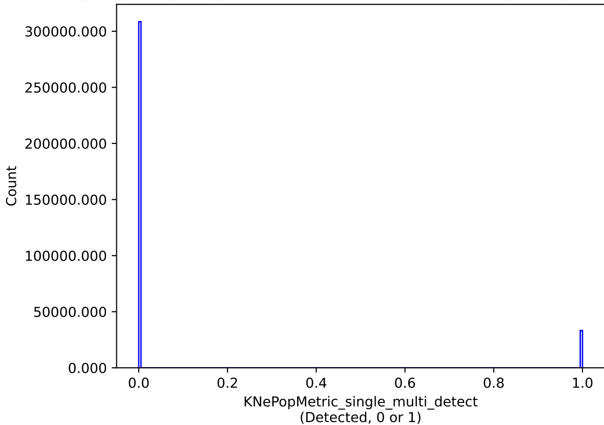
mw_roll_bulge_v3.3_10yrs single model: KNePopMetric_single_multi_detect
