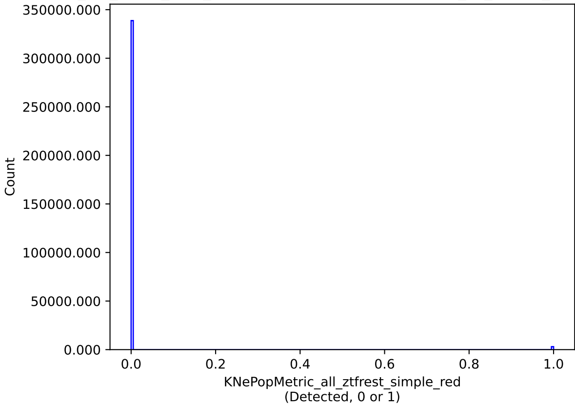
mw_roll_bulge_v3.3_10yrs all models: KNePopMetric_all_ztfrest_simple_red
