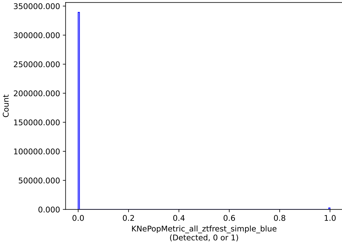
mw_roll_bulge_v3.3_10yrs all models: KNePopMetric_all_ztfrest_simple_blue
