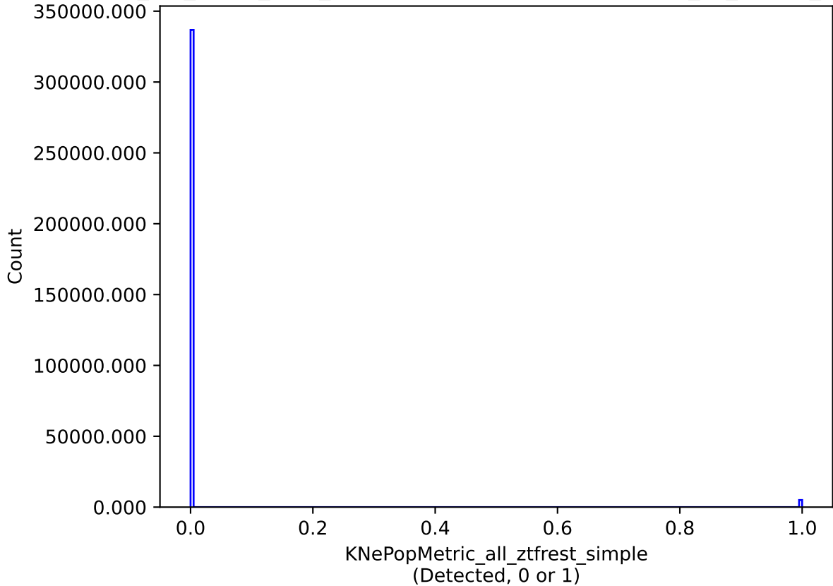
mw_roll_bulge_v3.3_10yrs all models: KNePopMetric_all_ztfrest_simple
