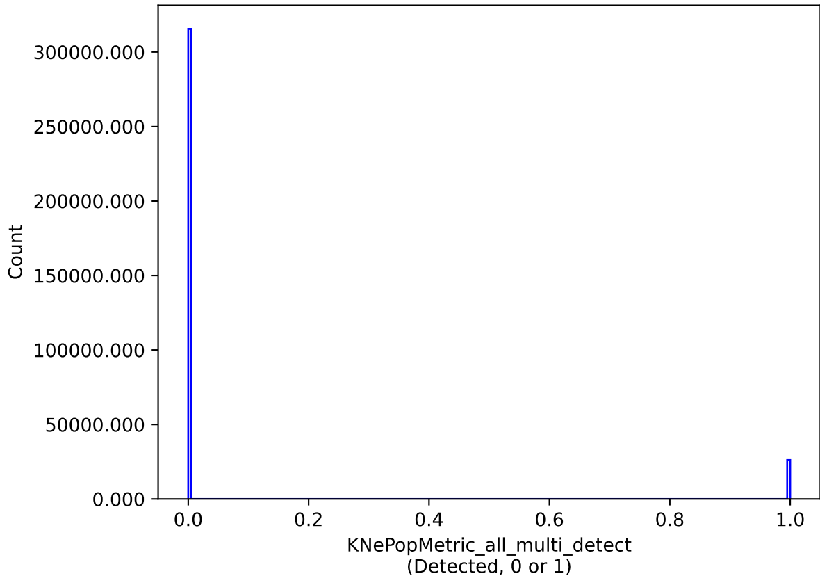
mw_roll_bulge_v3.3_10yrs all models: KNePopMetric_all_multi_detect
