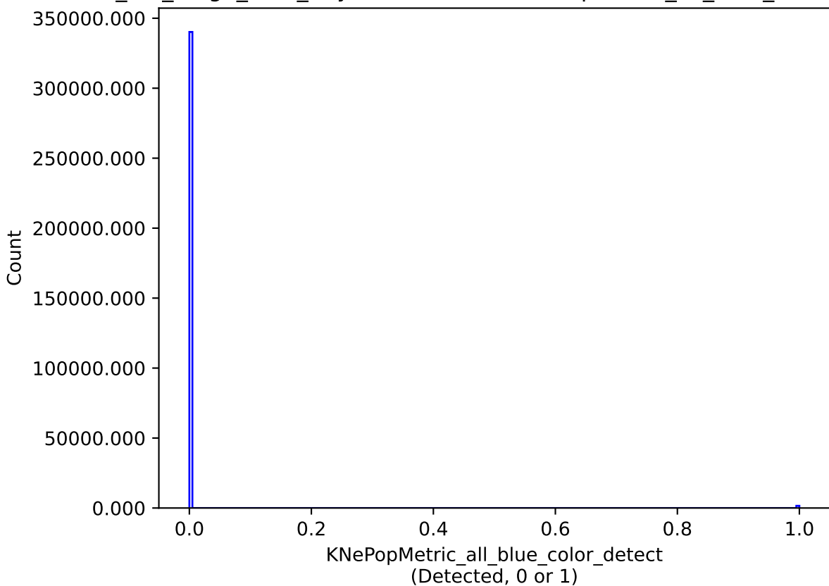
mw_roll_bulge_v3.3_10yrs all models: KNePopMetric_all_blue_color_detect
