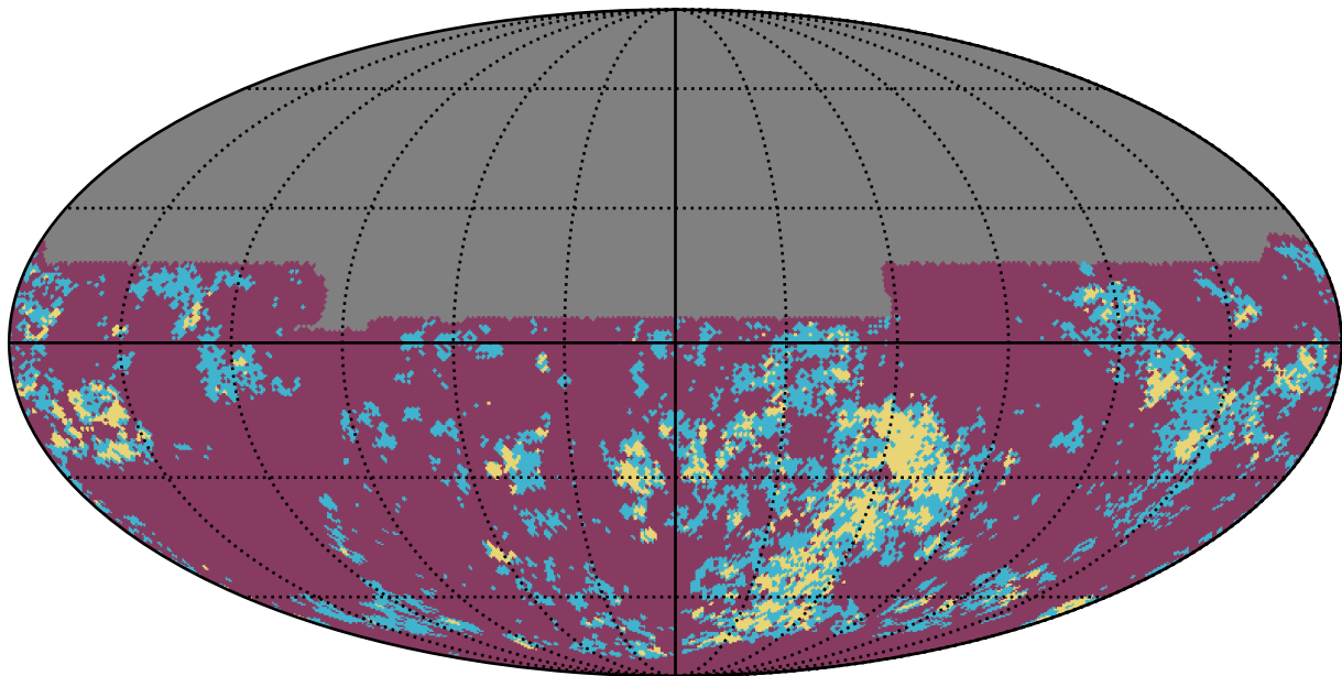
mw_roll_bulge_v3.3_10yrs y band: Gaps_7hr
