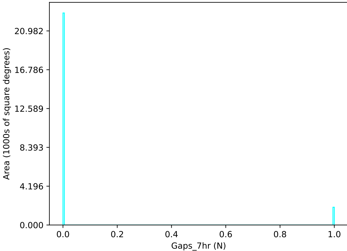
mw_roll_bulge_v3.3_10yrs u band: Gaps_7hr
