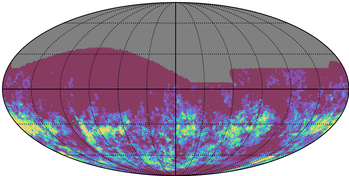
mw_roll_bulge_v3.3_10yrs r band: Gaps_7hr
