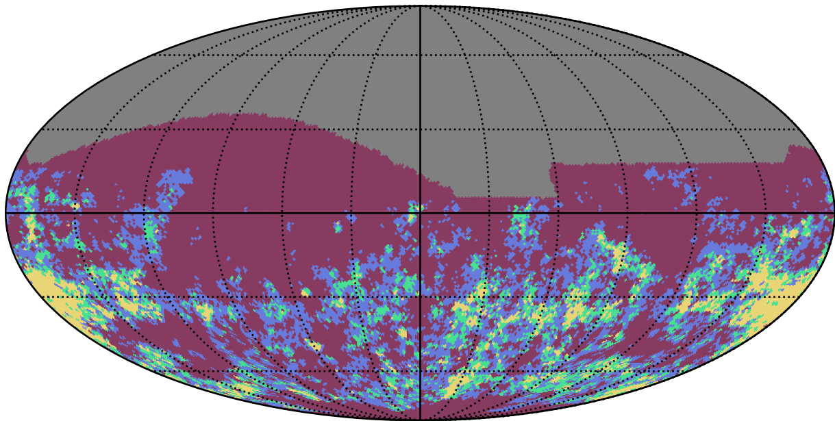
mw_roll_bulge_v3.3_10yrs i band: Gaps_7hr
