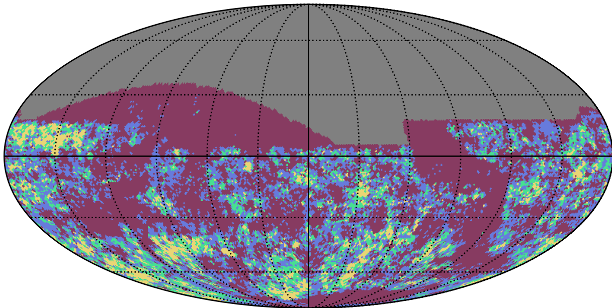
mw_roll_bulge_v3.3_10yrs z band: Gaps_3hr
