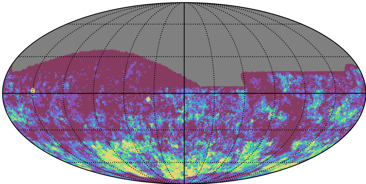
mw_roll_bulge_v3.3_10yrs r band: Gaps_3hr
