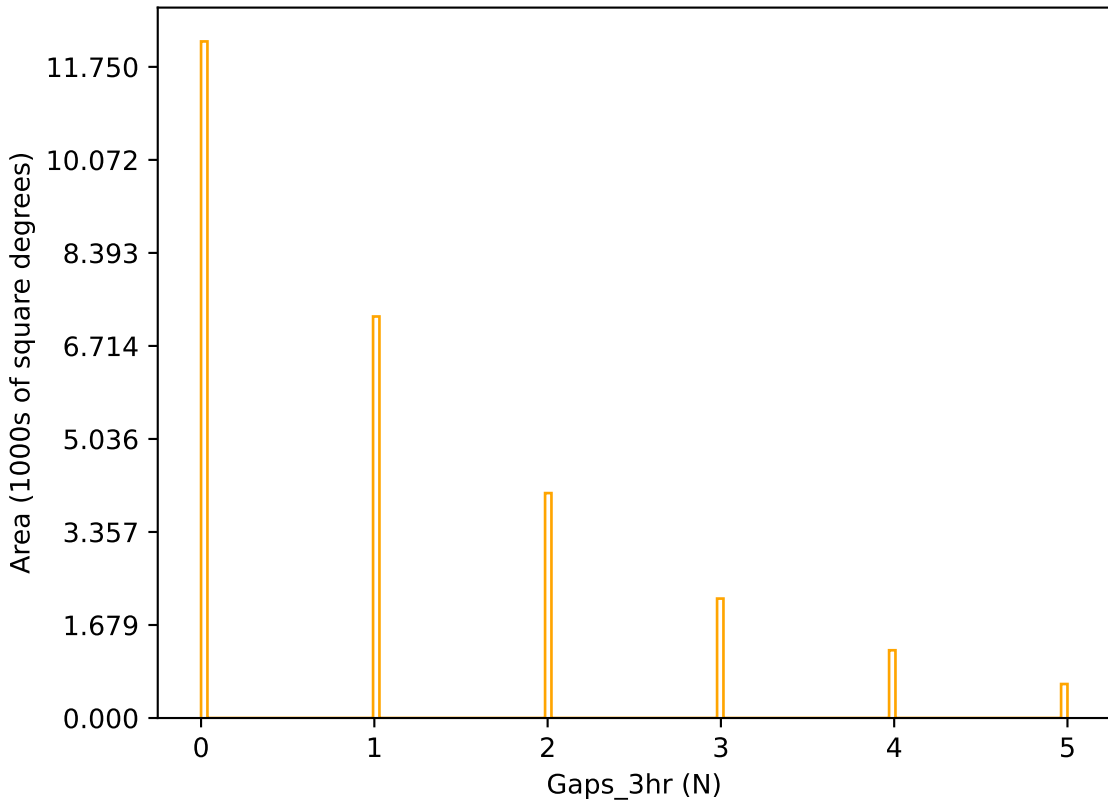
mw_roll_bulge_v3.3_10yrs r band: Gaps_3hr
