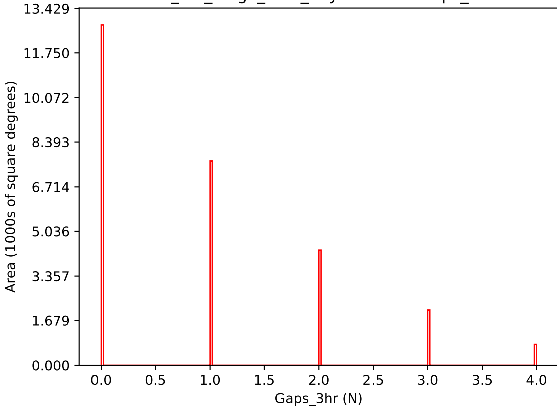
mw_roll_bulge_v3.3_10yrs i band: Gaps_3hr
