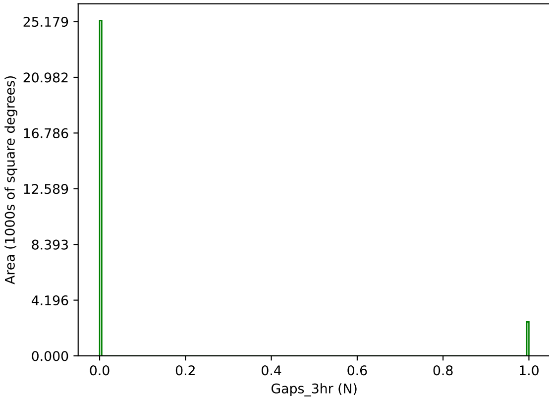
mw_roll_bulge_v3.3_10yrs g band: Gaps_3hr
