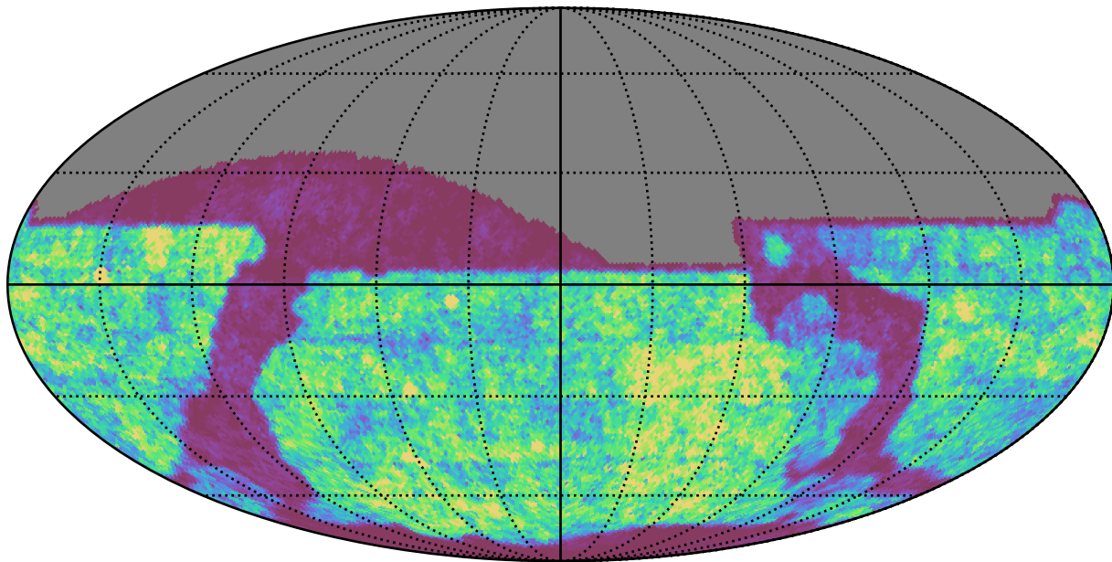
mw_roll_bulge_v3.3_10yrs z band: Gaps_24hr
