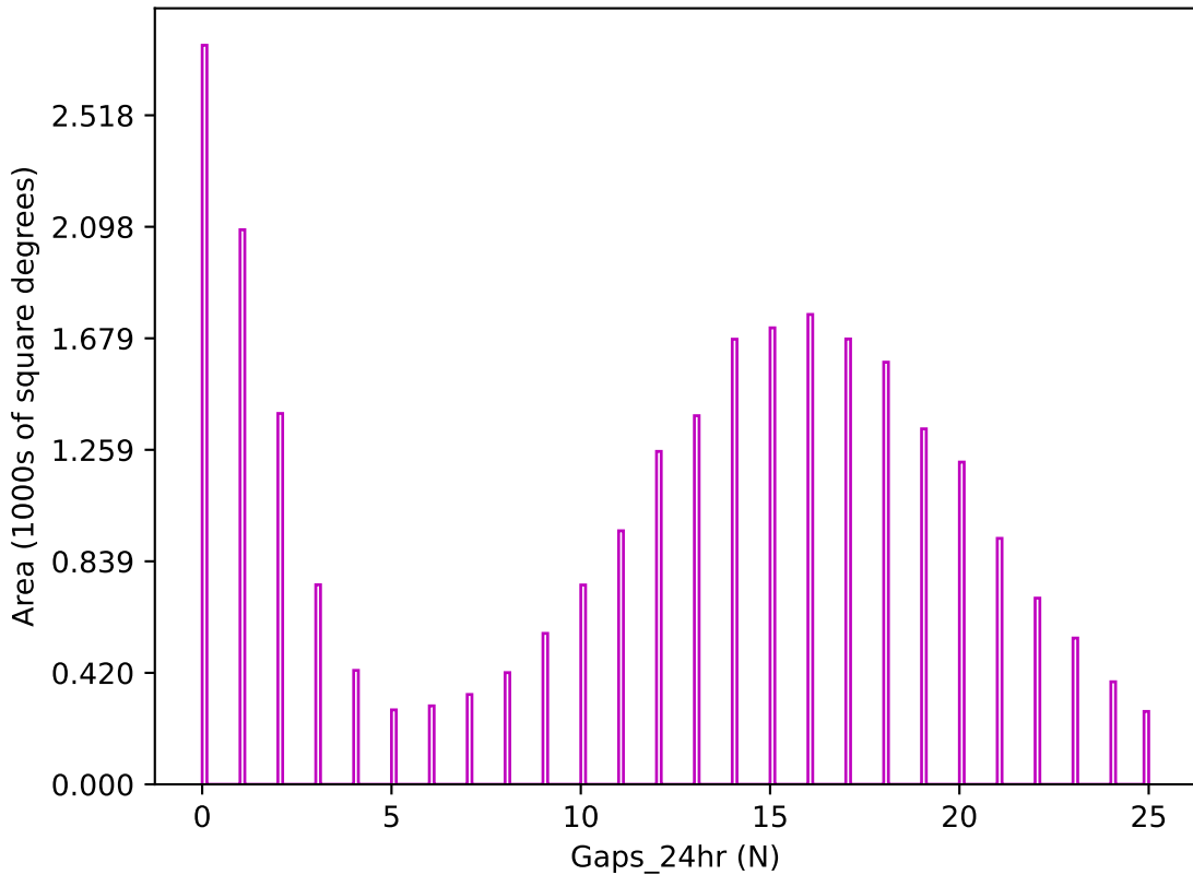
mw_roll_bulge_v3.3_10yrs z band: Gaps_24hr
