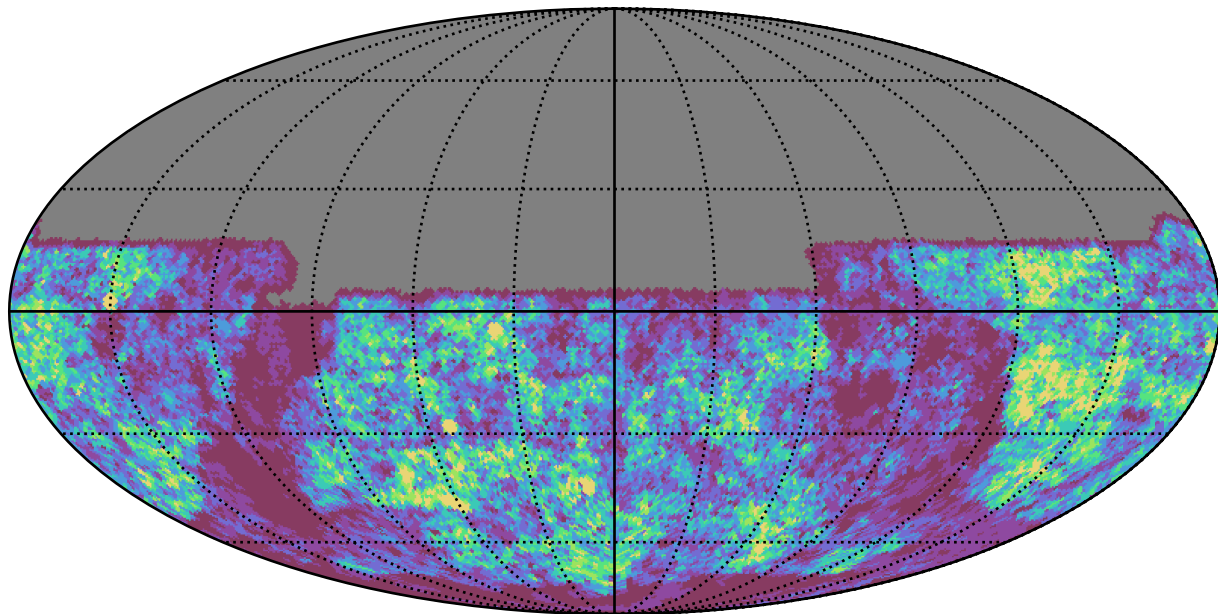
mw_roll_bulge_v3.3_10yrs u band: Gaps_24hr
