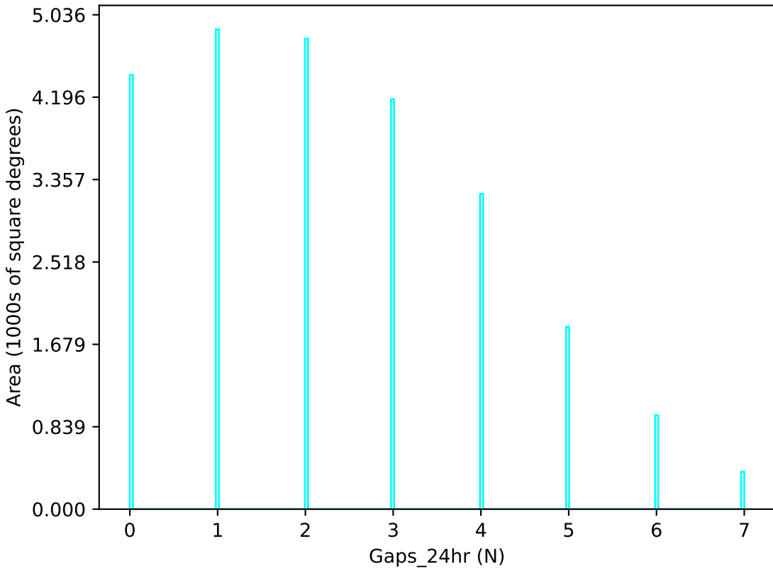
mw_roll_bulge_v3.3_10yrs u band: Gaps_24hr
