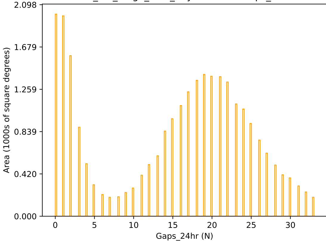
mw_roll_bulge_v3.3_10yrs r band: Gaps_24hr
