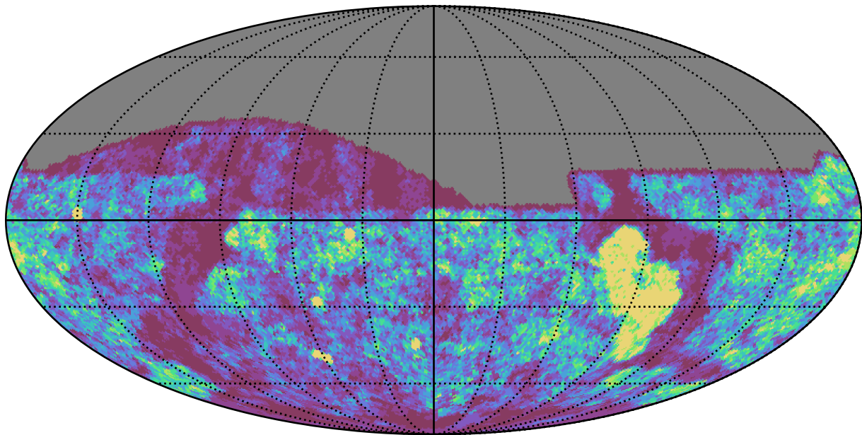
mw_roll_bulge_v3.3_10yrs g band: Gaps_24hr
