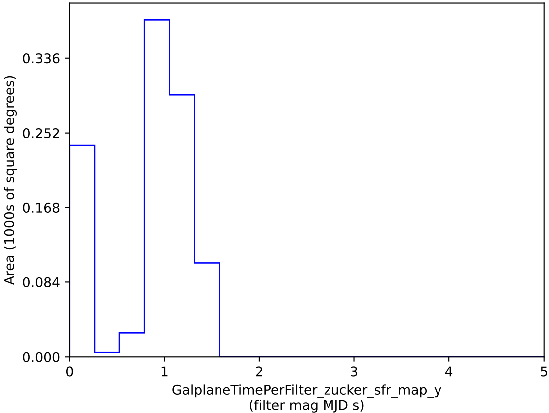
mw_roll_bulge_v3.3_10yrs : GalplaneTimePerFilter_zucker_sfr_map_y
