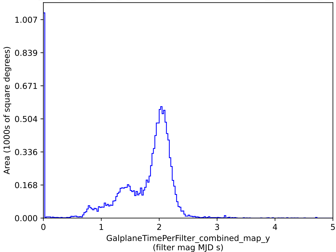
mw_roll_bulge_v3.3_10yrs : GalplaneTimePerFilter_combined_map_y
