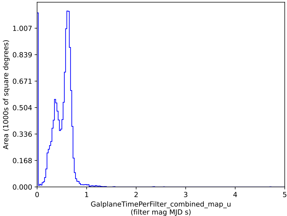
mw_roll_bulge_v3.3_10yrs : GalplaneTimePerFilter_combined_map_u
