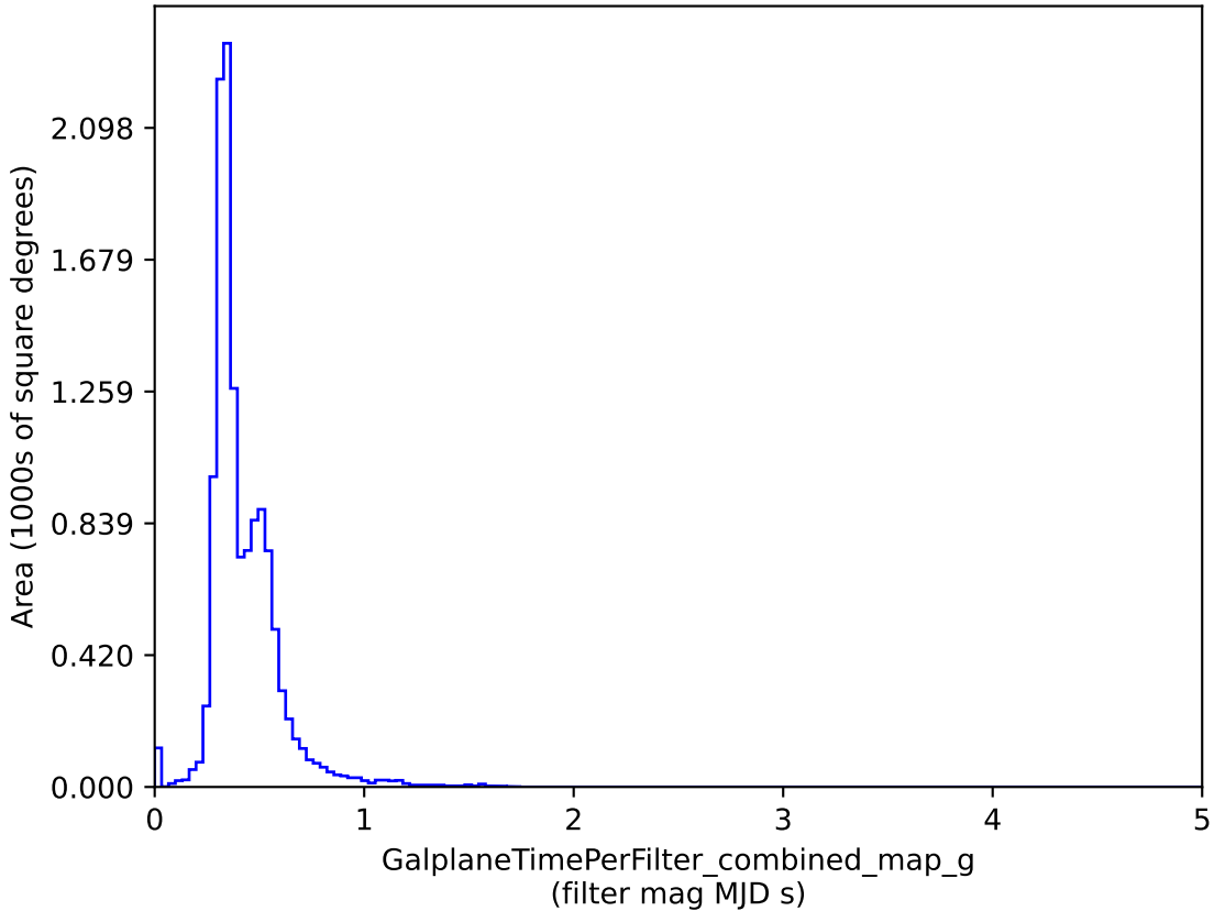
mw_roll_bulge_v3.3_10yrs : GalplaneTimePerFilter_combined_map_g
